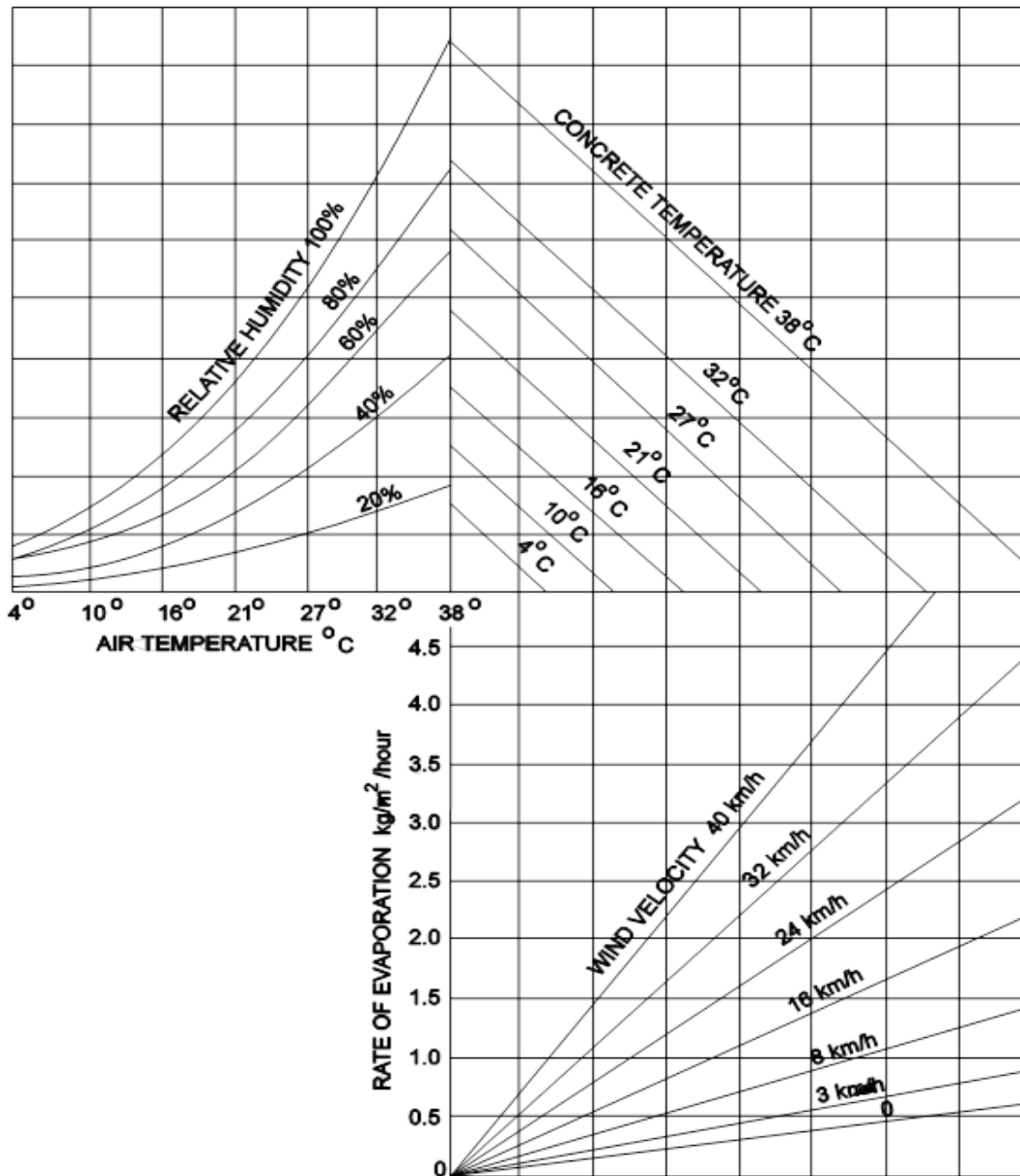
Figure 14.3: Evaporation from Concrete Freshly Placed on Site
