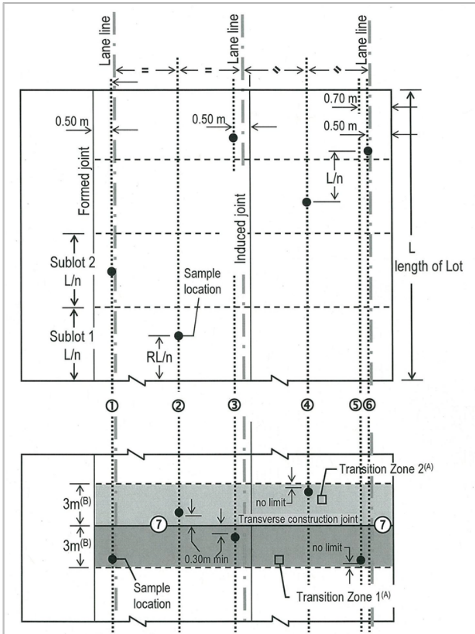
Figure 25.24: Sampling Locations for a Dual-lane Paving Sub-Lot
