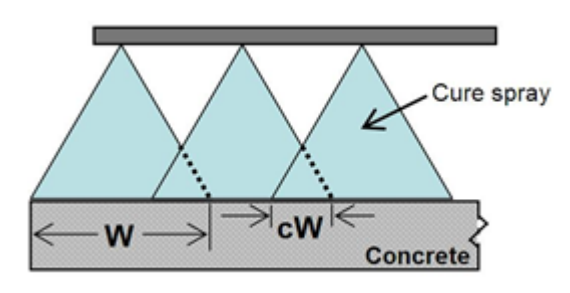
Figure 16.10: Curing Spray Overlap
