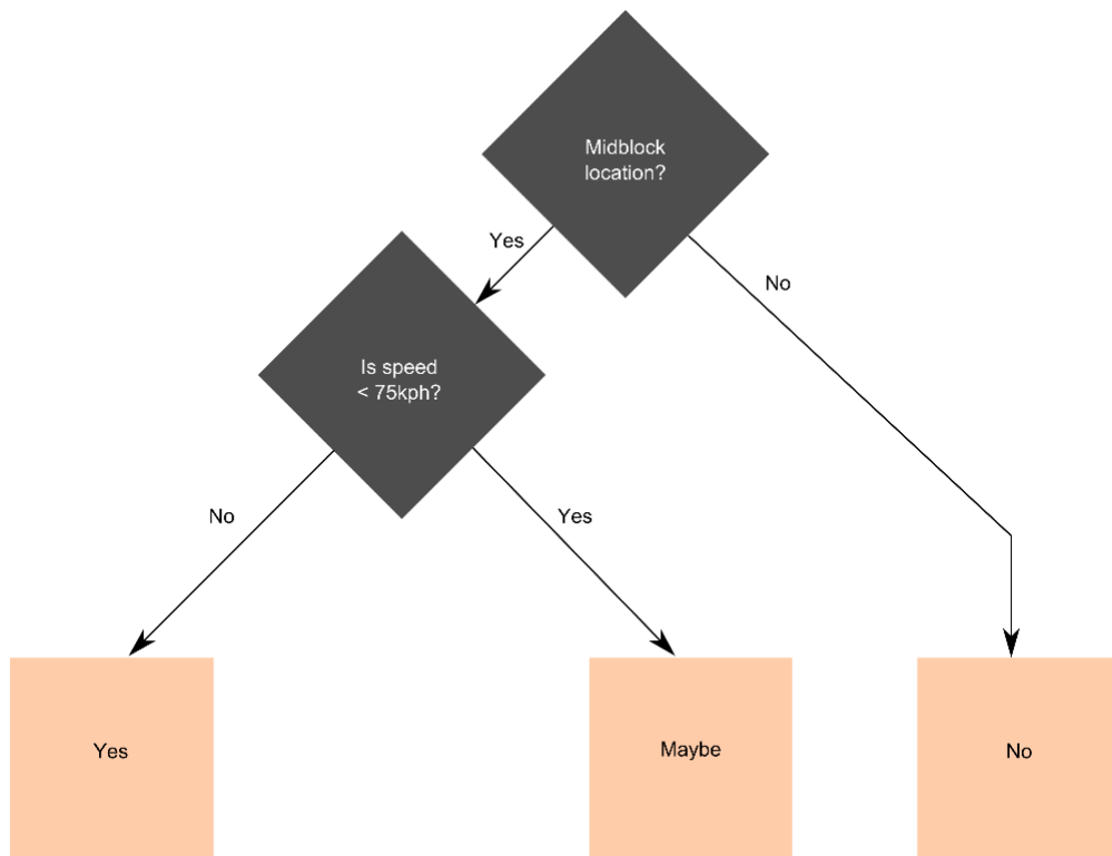
Figure 5. Grade separation feasibility decision tree
