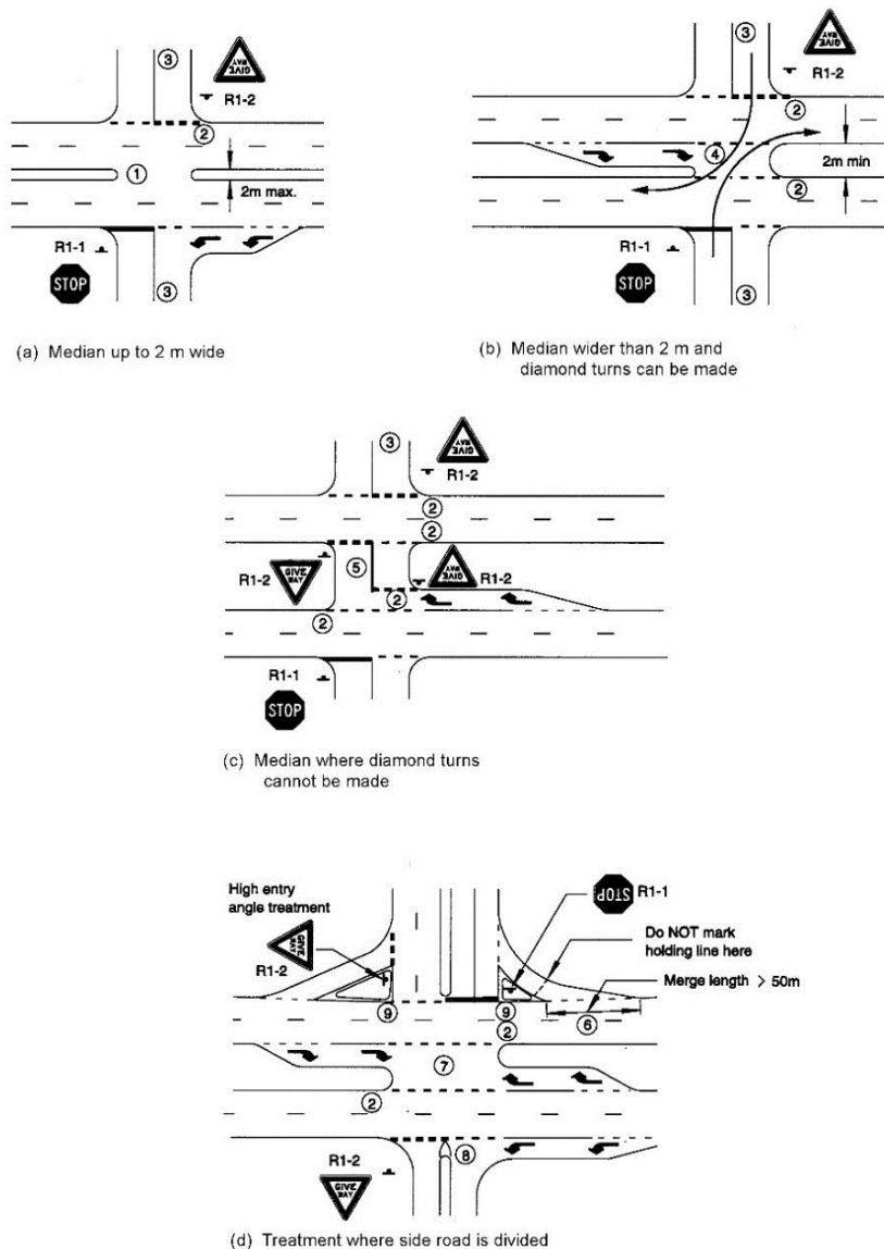
Figure 6.6: Typical stop line and give-way line treatments at kerbed intersections
