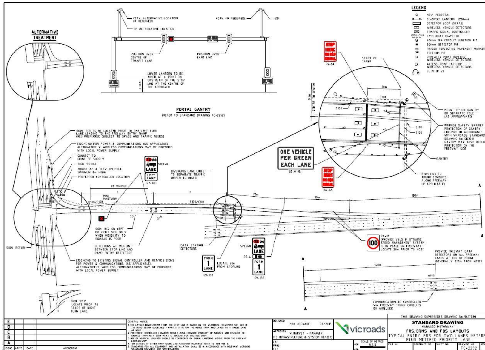
Figure 8.45: Typical freeway ramp signal for two lanes metered plus freeflow priority lane
