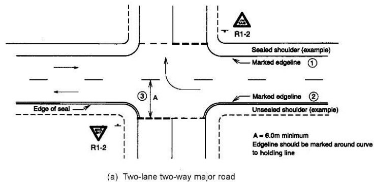
Figure 6.7: Typical give-way lines on roads that have shoulders
