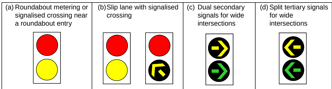
Figure 8.6: Two-aspect signal face layouts
