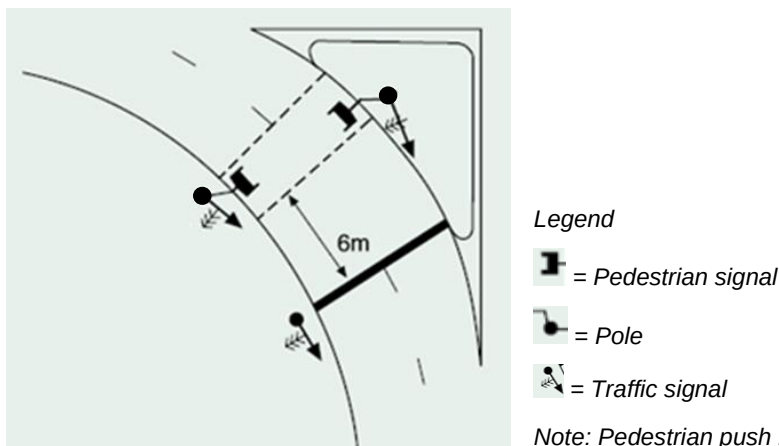
Figure 8.30: Signal face location for channelised left-turn control
