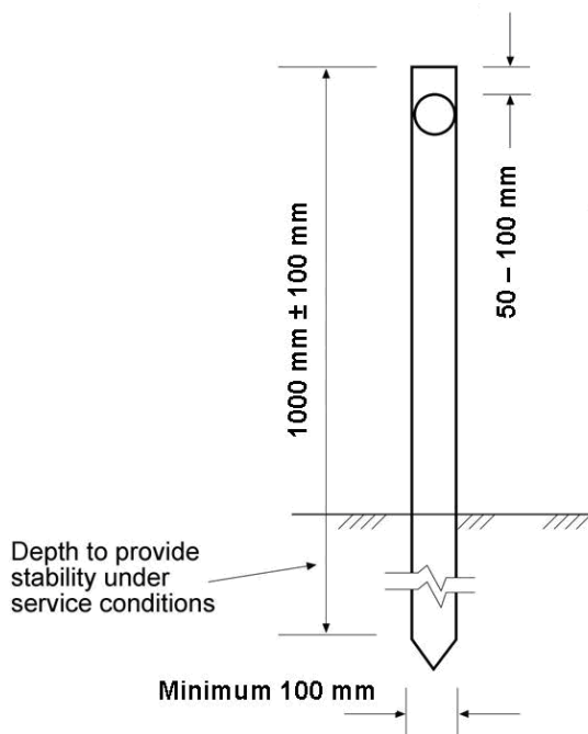
Figure 7.1: A typical guide post
