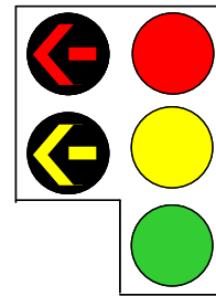
Figure 8.12: Five-aspect signal face layout with red and yellow left-turn arrow aspects
