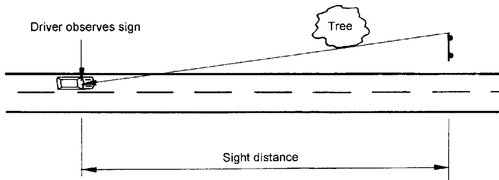
Figure B 1: Horizontal Sight Distance Measurement
