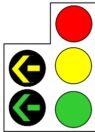
Figure 8.11: Five-aspect signal face layout with yellow and green left-turn arrow aspects
