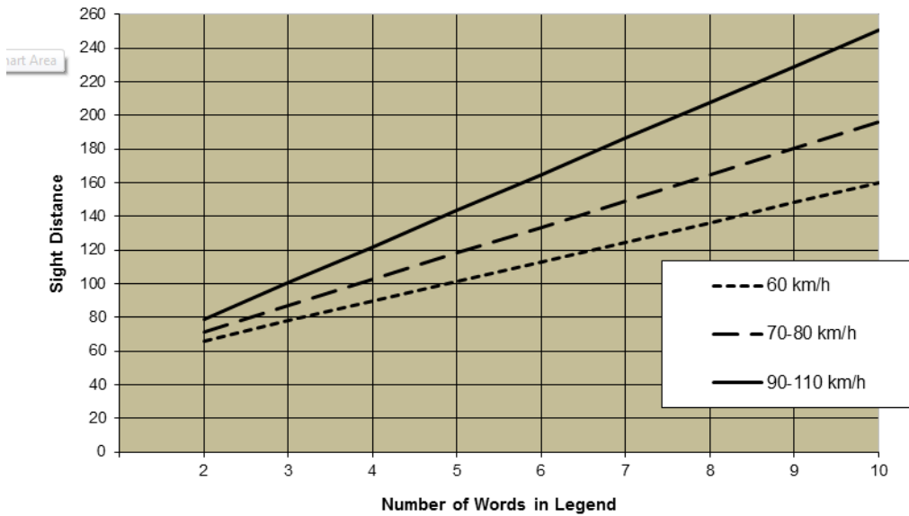
Figure B 3: Desirable Minimum Sight Distance Requirements
