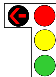
Figure 8.14: Four-aspect signal face layout with single left-turn red arrow aspect
