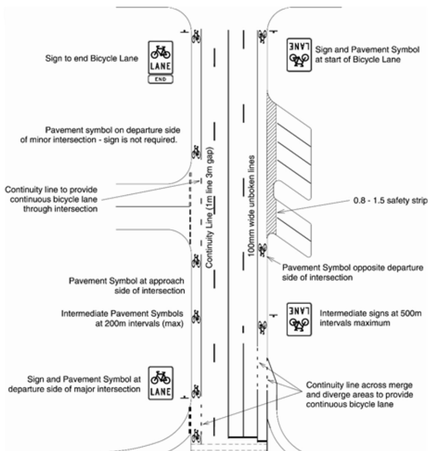
Figure 6.5: Example of bicycle-lane markings
