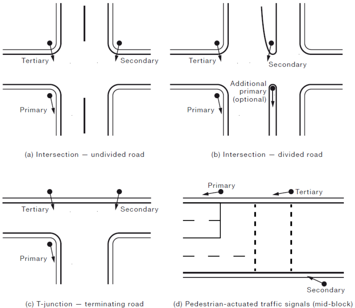
Figure 8.28: Designation of signal faces
