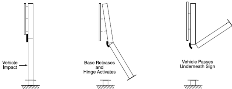
Figure C1 1: Impact performance
