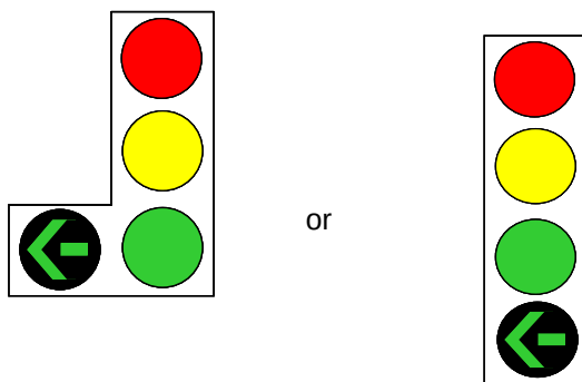
Figure 8.13: Four-aspect signal face layout with single left-turn green arrow aspect
